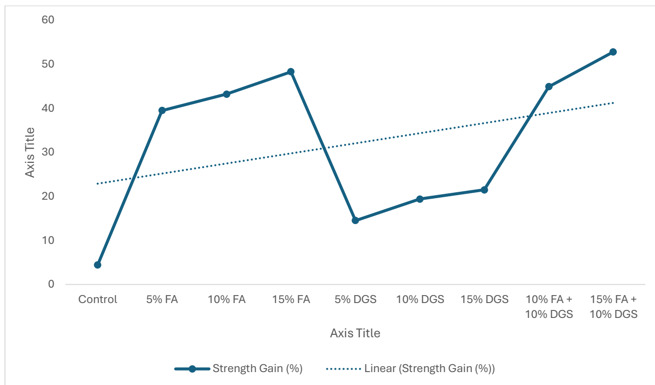
Figure 4: Strength gain after 28 days
