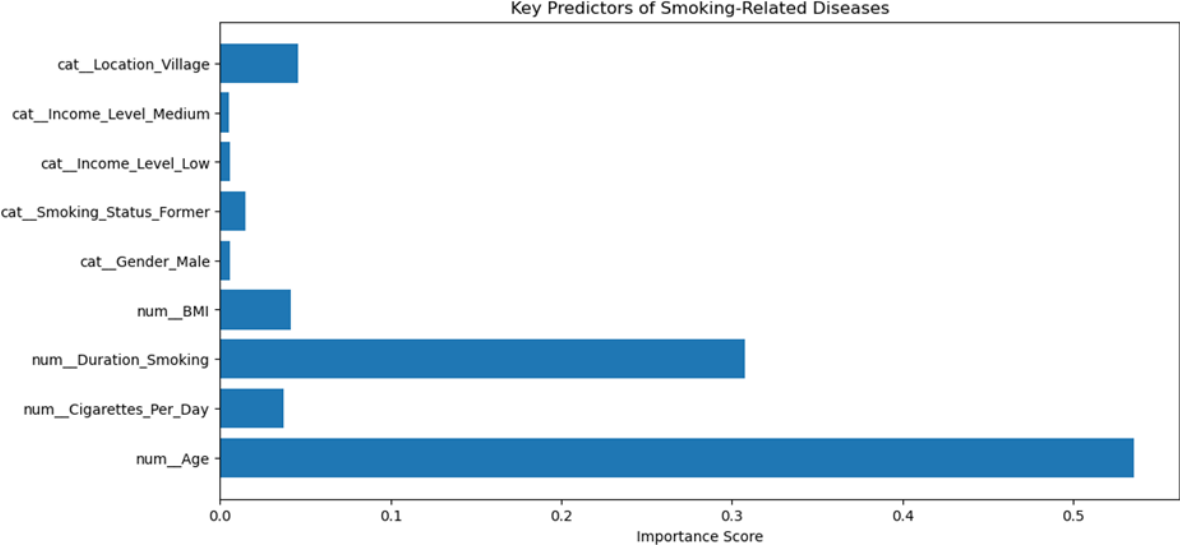
Figure 9: Key Predictors
