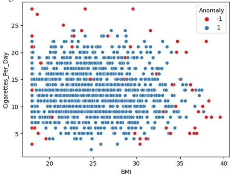
Figure 7: Anomaly Detection
