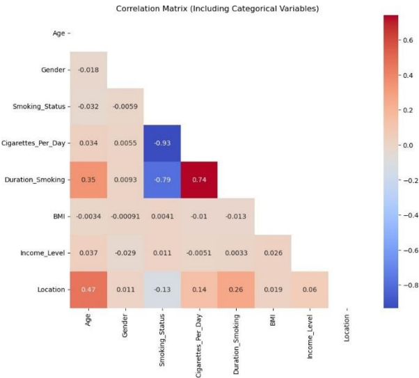
Figure 4: Correlation Analysis
