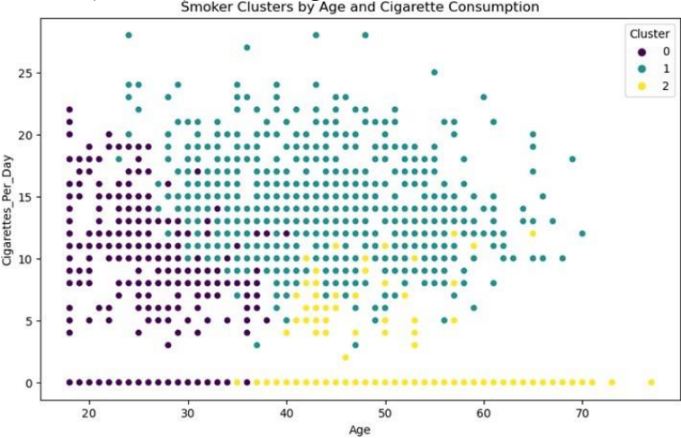
Figure 8: Smoker Clustering
