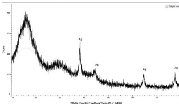
Fig.3. XRD pattern of synthesized SiAg NCs with linker, MPTMS (SiAg-M)
