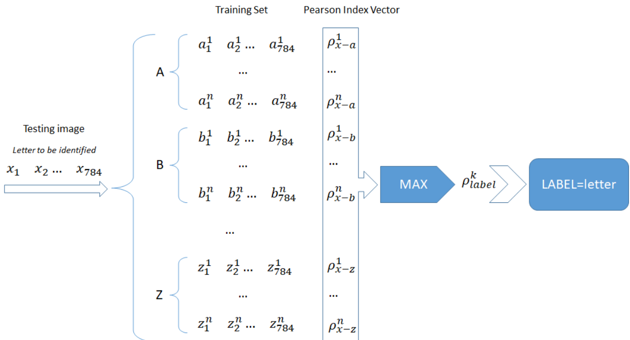
Figure 6 Algorithm for Letter identification
