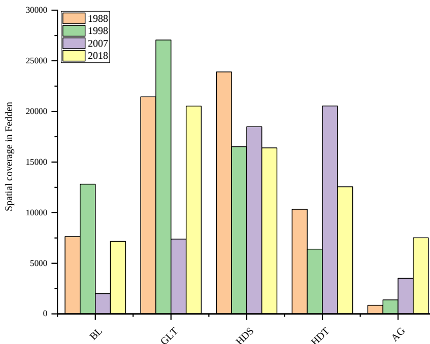
Fig. 4. Spatial coverage of different classes in EL-Rawashda forest from 1988 to 2018.
