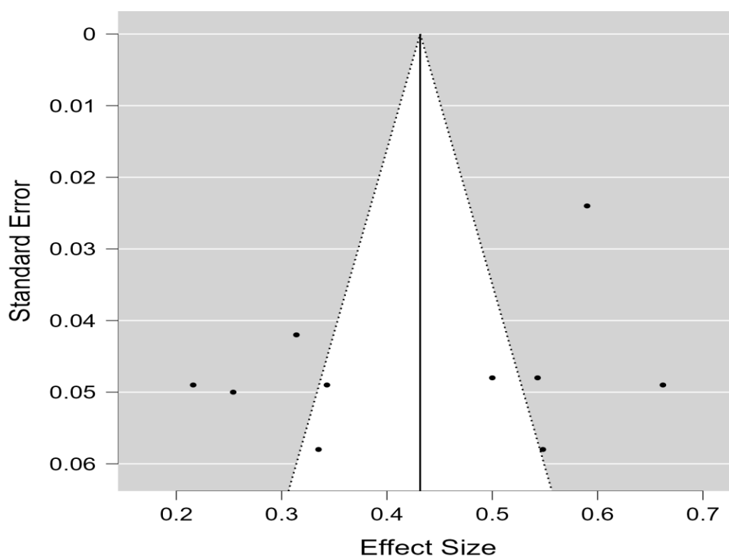
Fig 3. Funnel Plot
