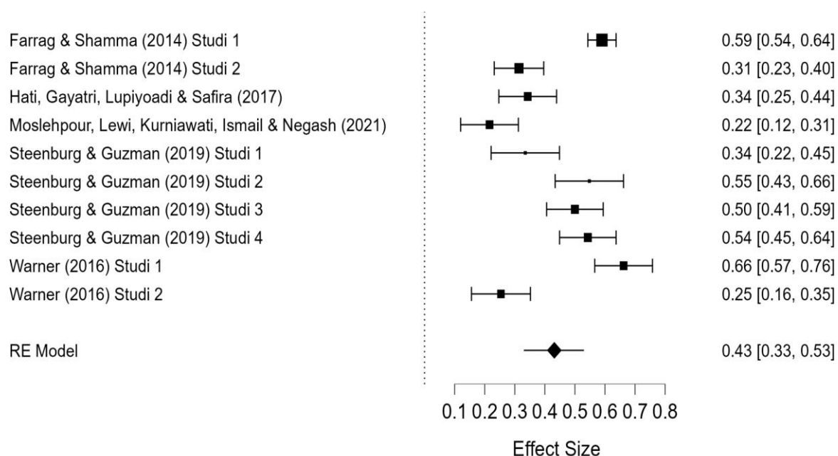
Fig 2. Forest Plot
