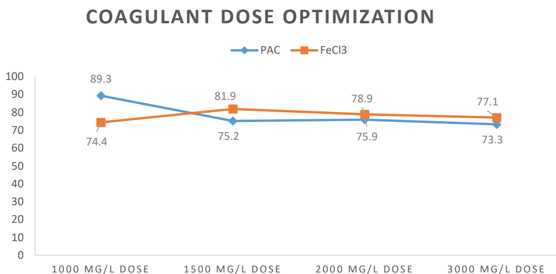
Figure 4: COD reduction in % through coagulant dose optimization
