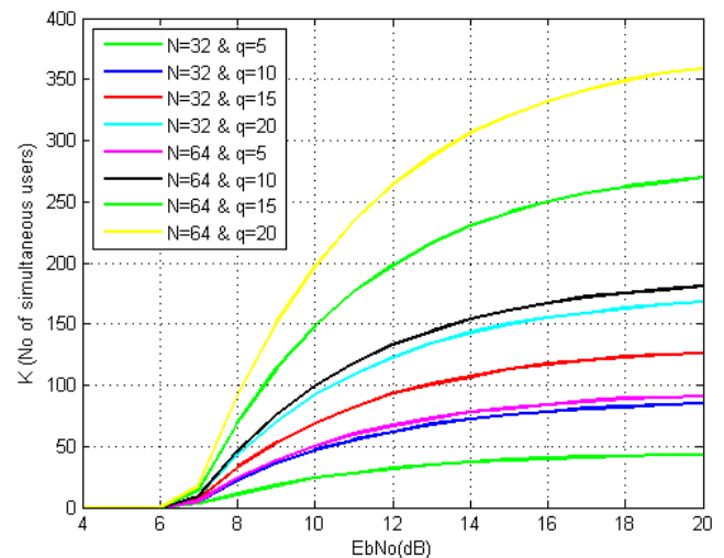
Fig. 7. Multiple Access Capability of System for varying different Network Parameters
