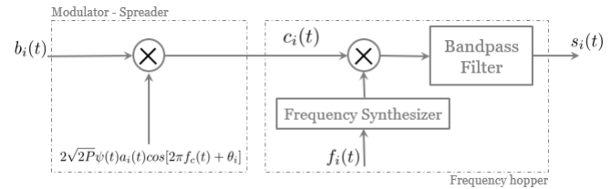
Fig. 1. H-SSMA System - Transmitter Model
