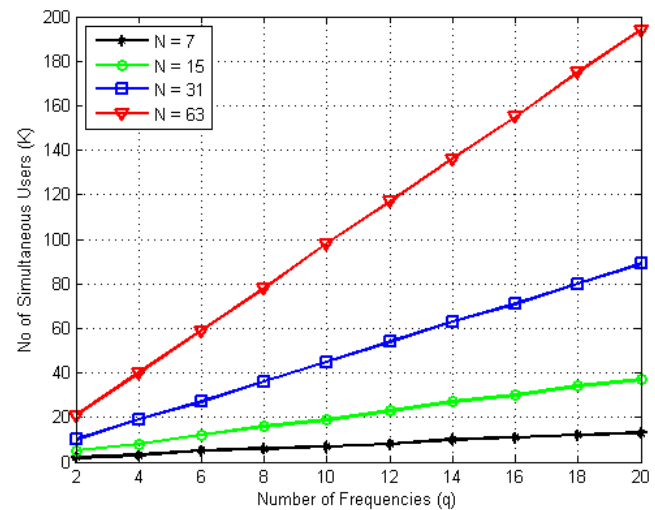
Fig. 4. K as a function of q for various Code Lengths
