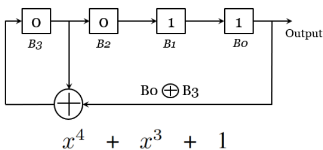
Fig. 8. LFSR - Feedback Connection Formation
