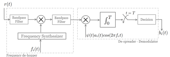
Fig. 2. H-SSMA System - Receiver Model
