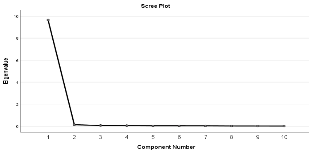
Figure 6: Scree Plot
