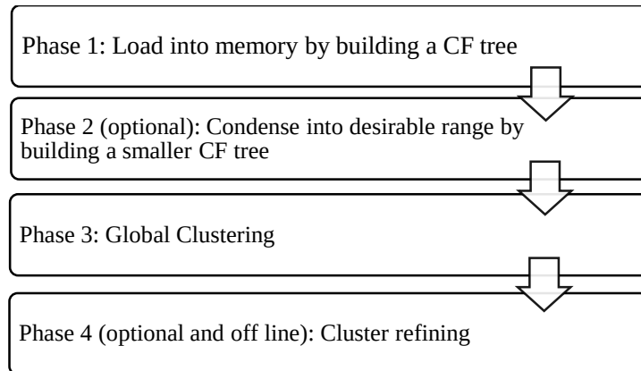
Figure 3.1.1. BIRCH Algorithm Overview
