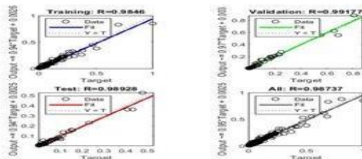
Figure 6c: Regression analysis the Model
