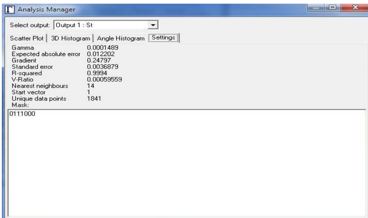
Figure 5: Mask Result of Input variables from Genetic Algorithm
