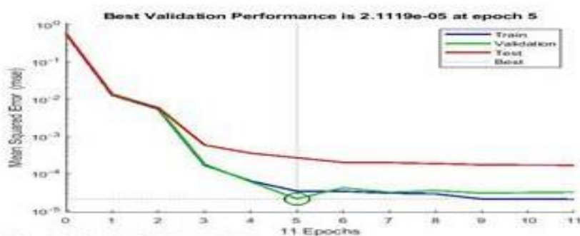
Figure 8b: the plot of MSE against Epoch
