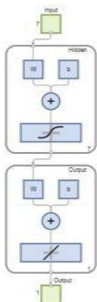
Figure 7a: ANN Architecture
