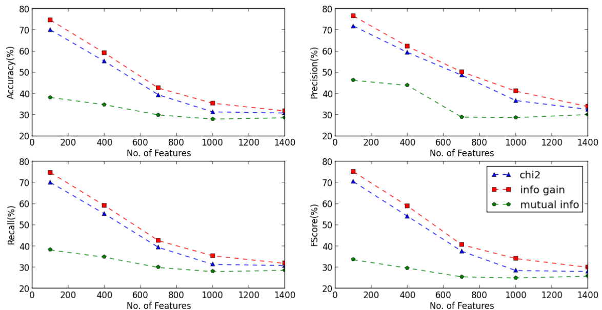
KNeighborsClassifier
