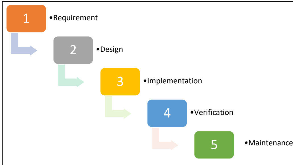
Fig. 1. : Waterfall Model
