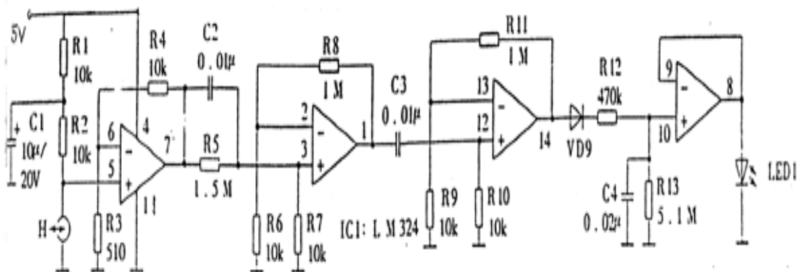
Figure 2. Magnetic detection circuit
