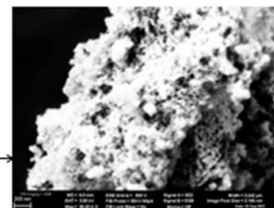
From SEM results of the TiO 2 -Ag composite prepared with chitosan (Fig 3.a), it can be deduced that many impurities are contained and the titania particles with and without pores embedding Ag are spreading inconsistently. Fig.3(b) shows the micrographs of Ag-TiO 2 nanocomposites prepared without chitosan as stabilizing agent. As it is clearly indicated from the presented micrographs, the aggregated growth of spherical particles with the presence of metallic silver on mesoporous surface of the TiO 2 nanoparticles can be seen. And also some TiO 2 particles without pores and Ag are observed. The obtained composition is in good agreement with the experimental result from XRD analysis.
