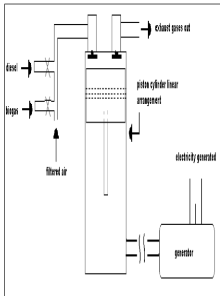
FIG.1.5 DUAL FUEL
