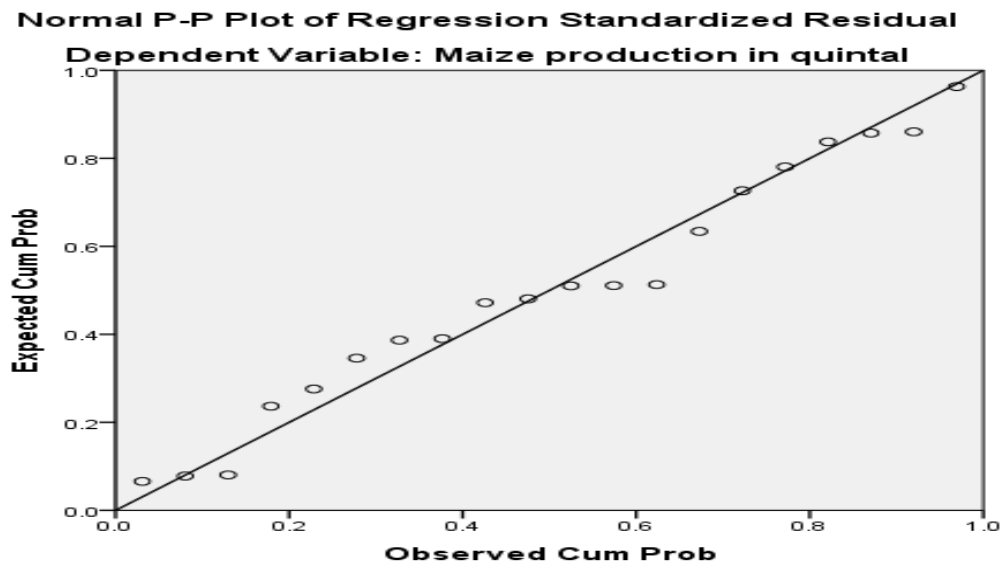
Figure 2: Normal P-P plot for assumption of linearity checking
