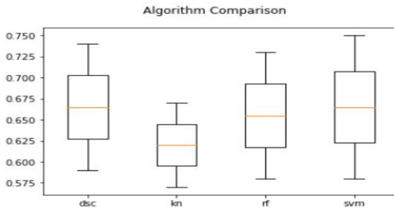
Figure 8: algorithm comparison
